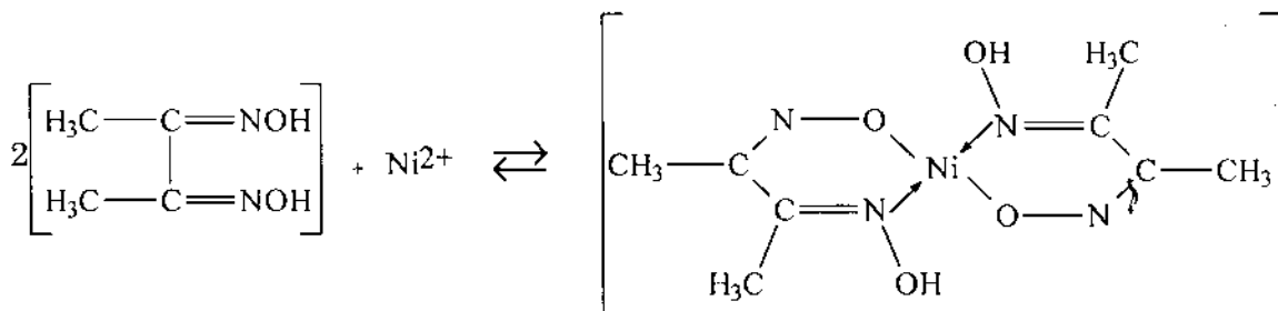
Dimethylglyoxin
