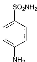
Sulfanilamid
