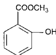
Methyl salicylac
