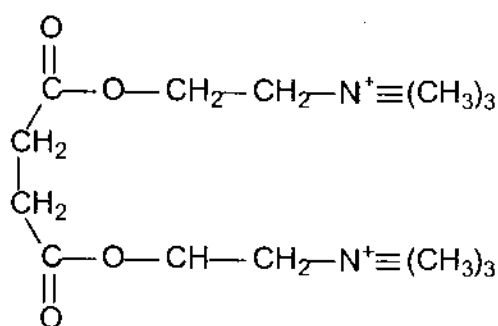
Succinylcholin
