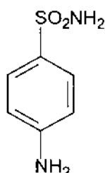
Sulfanilamid
