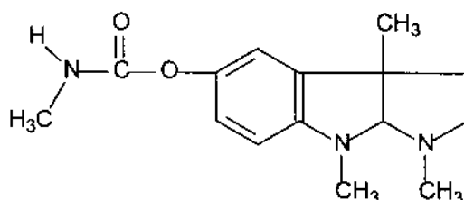
Physostigmin
