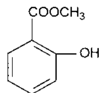
Acid salicylic
