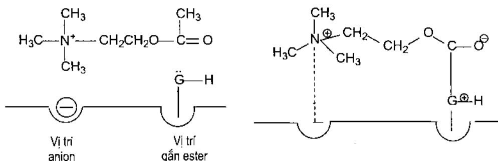
Cholinesterase
