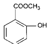
Acid salicylic
